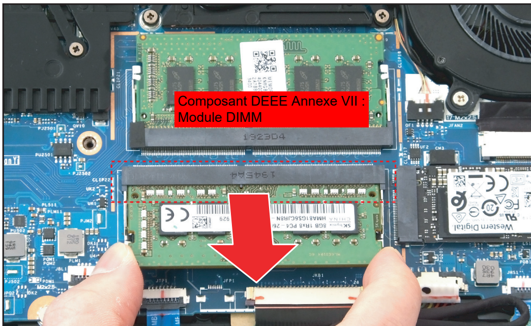
Figure 1-12. Retirer le module DIMM
