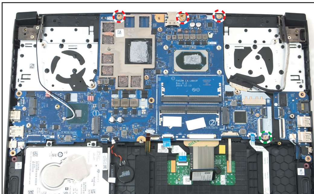
Figure 1-27. Retirer les vis
