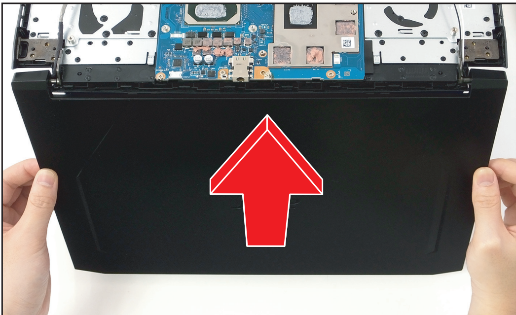
Figure 1-21. Retirer le module LCD
