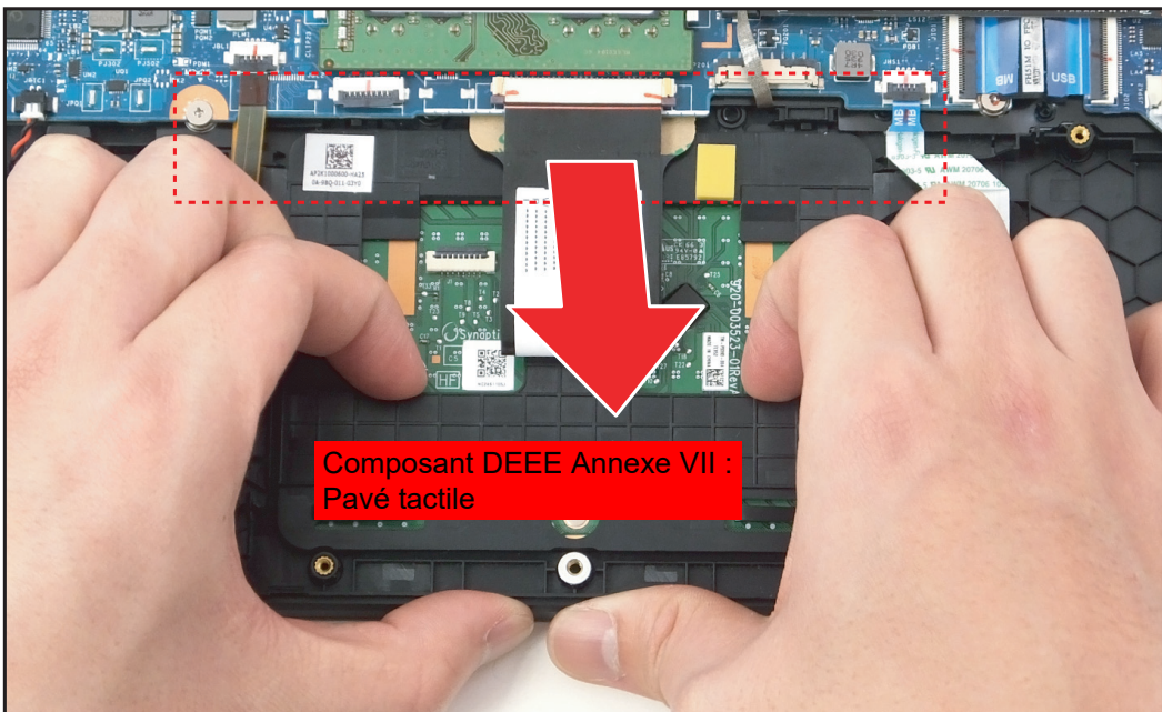
Figure 1-35. Retirer le pavé tactile
