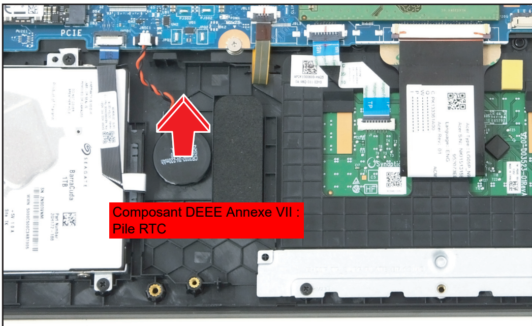
Figure 1-31. Retirer la pile RTC
